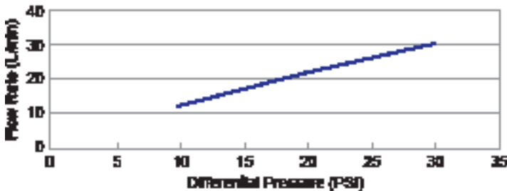
Clean Water Flow Rate 10" Segment (4)
